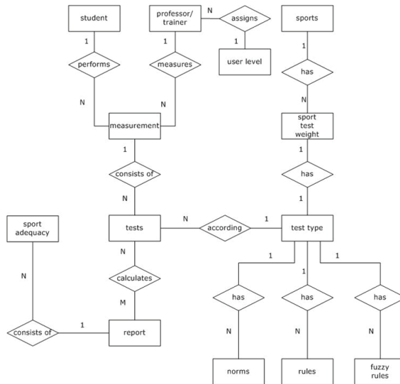
Fig. 5. Expert system structure. Expert knowledge is stored as rules, norms and test weights for each sport.
