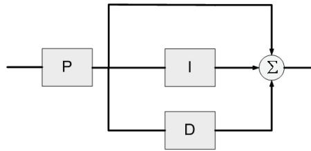
Fig. 2. PID regulator in standard topology
