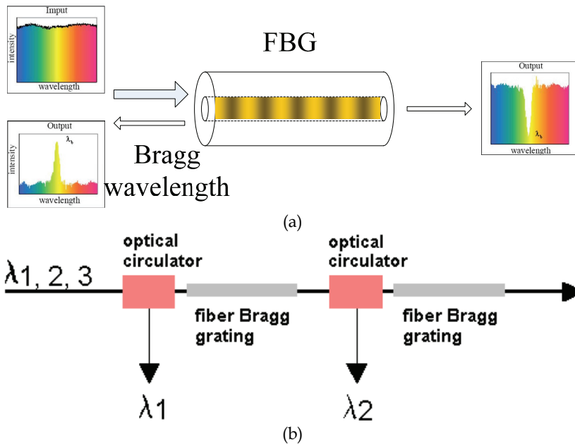
Fig. 25. Fiber Bragg gratings principle of operation for single and serially placed gratings.
