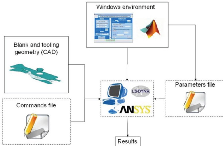
Fig. 4. Automation procedure
