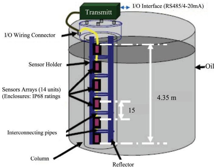
Fig. 11. Hardware overview
