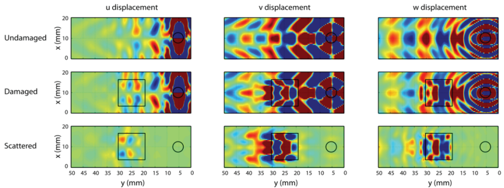
Fig. 24. Simulation results for longitudinal (u,v) and transverse (w) displacement components on the surface of a metallic structure ( undamaged case (top), damaged area (middle) and scattered field (bottom)).
