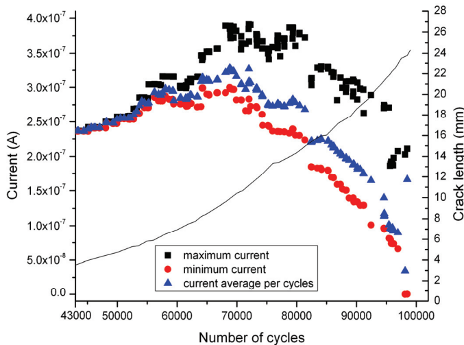
Fig. 15. Crack growth monitoring using CNT-based sensor.
