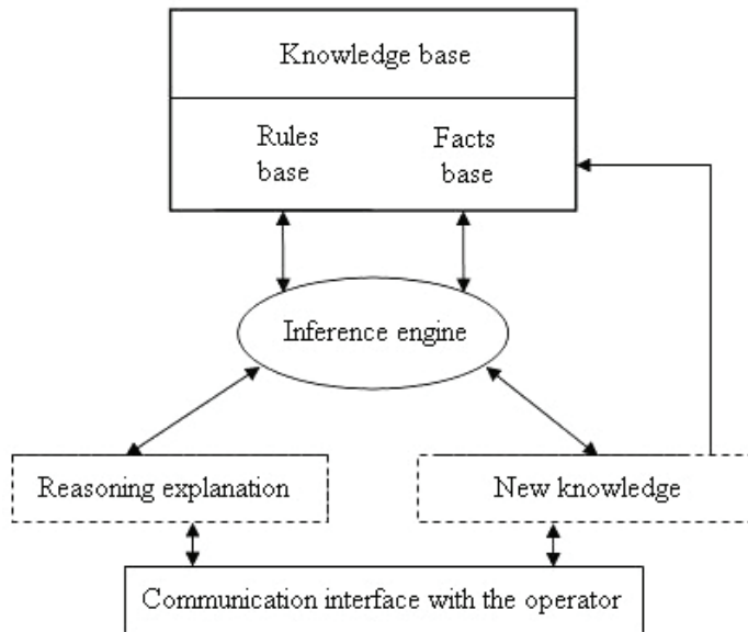
Fig. 6. General structure of an ES.
