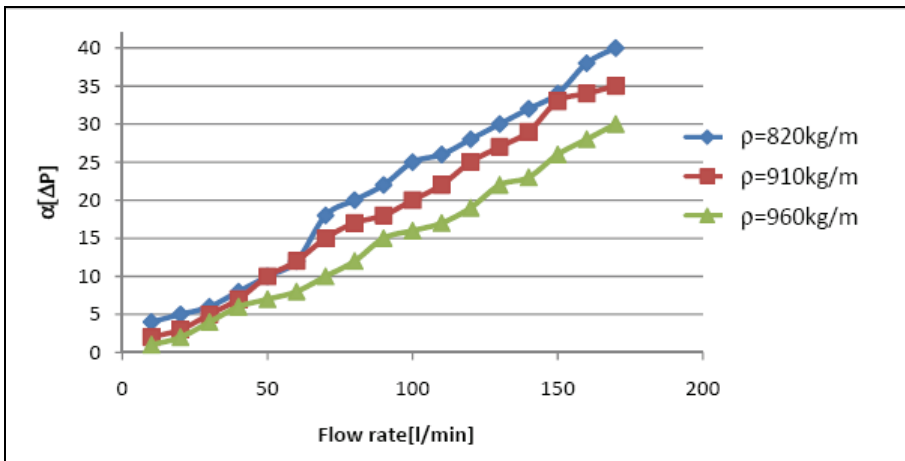
Fig. 16. Differential pressure versus flow rate for various liquid densities
