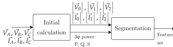
Fig. 5. Segmentation and feature extraction.
