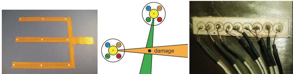
Fig. 23. Schematic of sensors/actuators network Layout (Acellent SMART layer, Metis Design Intelliconnector & Vector locator, and university of Sherbrooke’s micro-machined PZT array).
