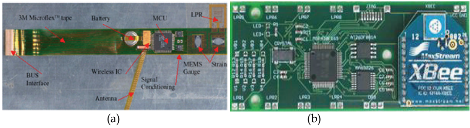
Fig. 17. Smart MEMS based smart sensor node.
