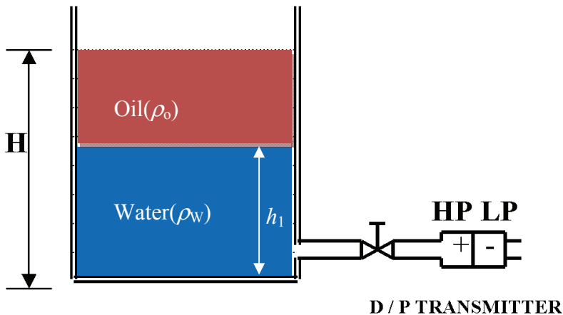
Fig. 1. Principle of interface level measurement using pressure sensors.
