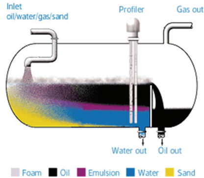
Fig. 7. The Nucleonic Tracerco's level measurement system ([18,19]).
